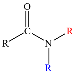
Amide group
