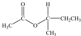
1-methylpropylethanoate
