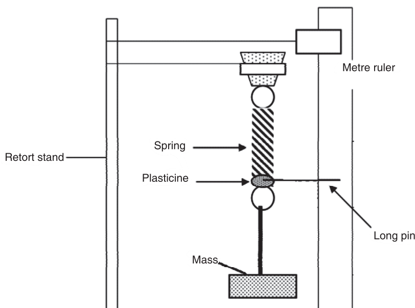
Fig.2-4; Oscillation of a mass on spring
