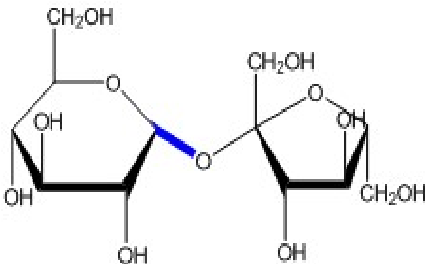
b monosaccharide monosaccharide disaccharide
