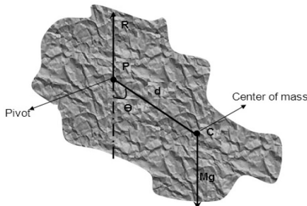
Fig.2-2; Compound pendulum
