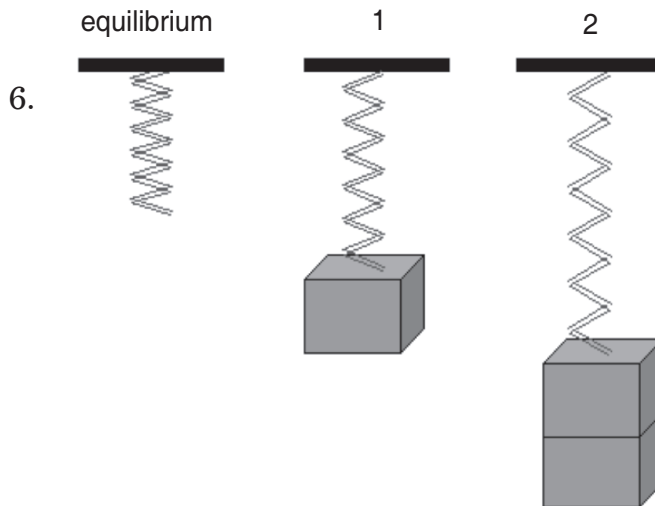
Fig.2-2; Helical springs
