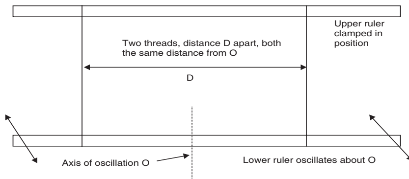
Fig.2-3; Bifilar suspension
