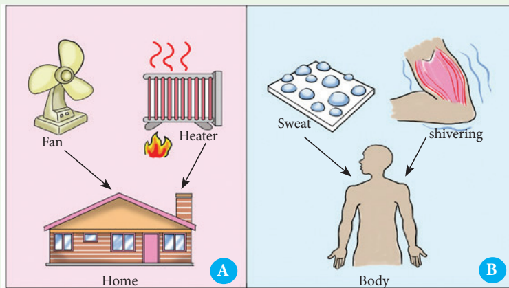
Fig. 10.1: Temperature control
