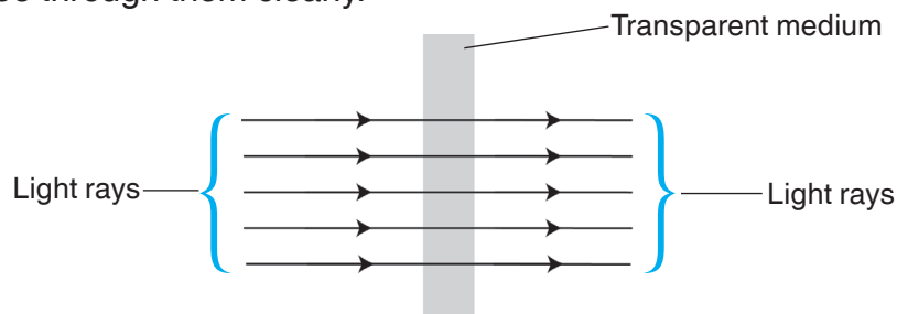
Fig. 14.1: Transparent medium.
