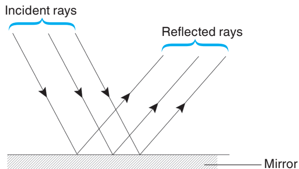
Fig. 14.5: Regular reflection.
