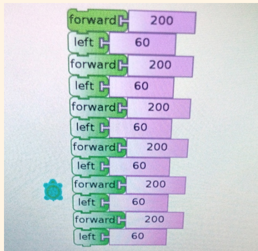
Turtle Commands.
