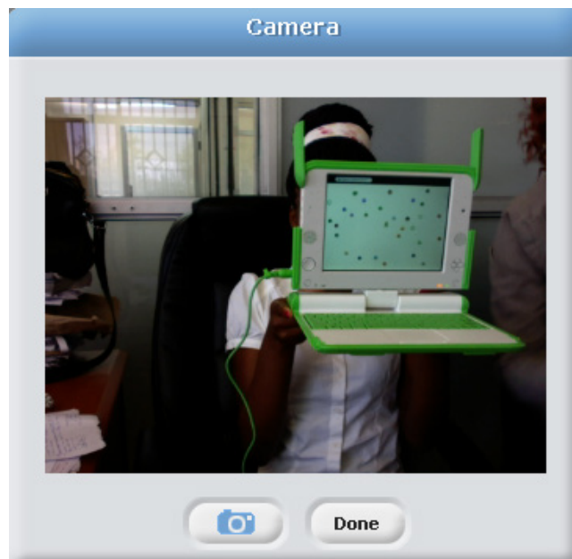
Fig. 7.16: Camera Sprite.
