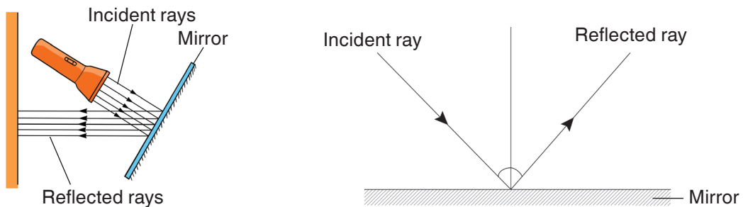
Fig. 14.4: Reflection of light.
