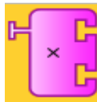
Fig. 7.10: Multiplication operation.
