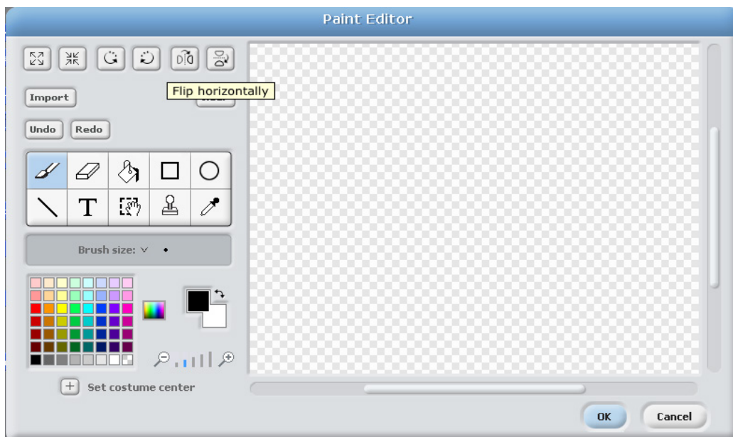
Fig. 7.14: Paint Option.
