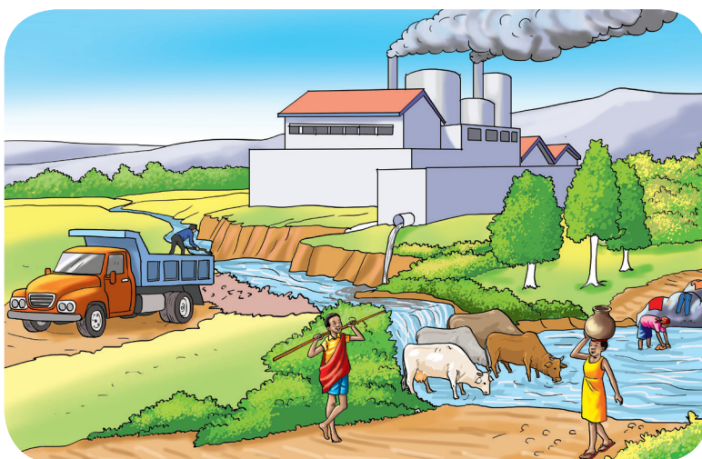
Fig 8.11 Water pollution.
