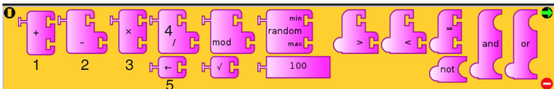
Fig. 7.5: Arithmetic operations.
