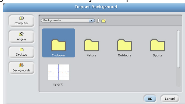
Fig. 7.20: Import option.
