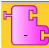
Fig. 7.8: Subtraction operation.
