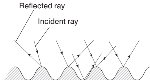
Fig. 14.6: Irregular reflection.
