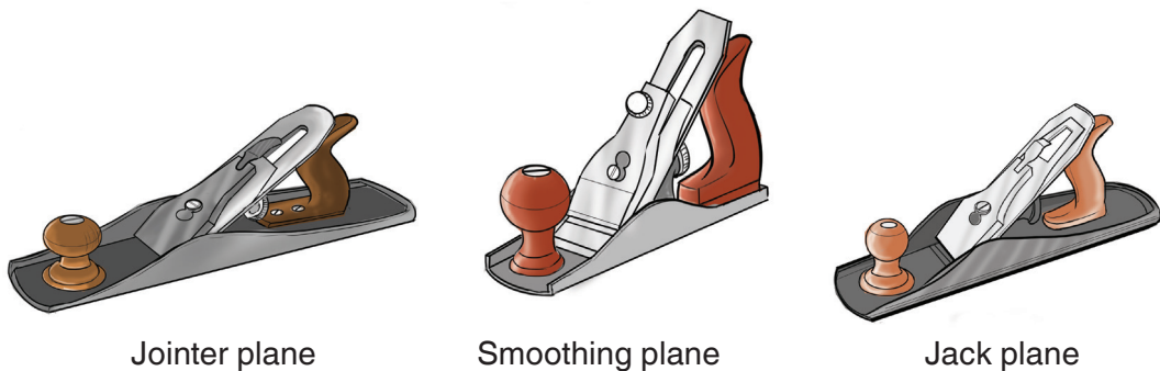
Fig 1.5: Types of planes
