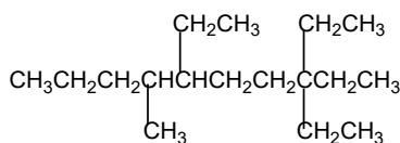
3,3,6-triethyl-7-decane
