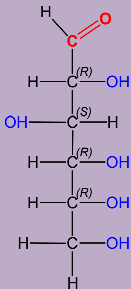
Glucose
