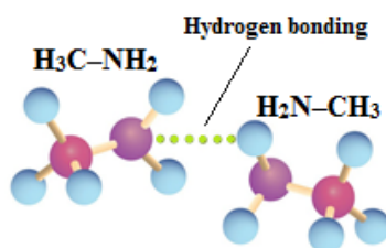
Figure 9.1. Hydrogen bonding between two amine molecules
