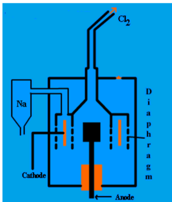
Figure 13.8.1: Down cell
