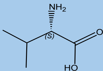
valine
