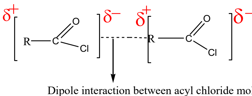
Figure 7.9. Intermolecular forces between molecules of acyl chlorides
