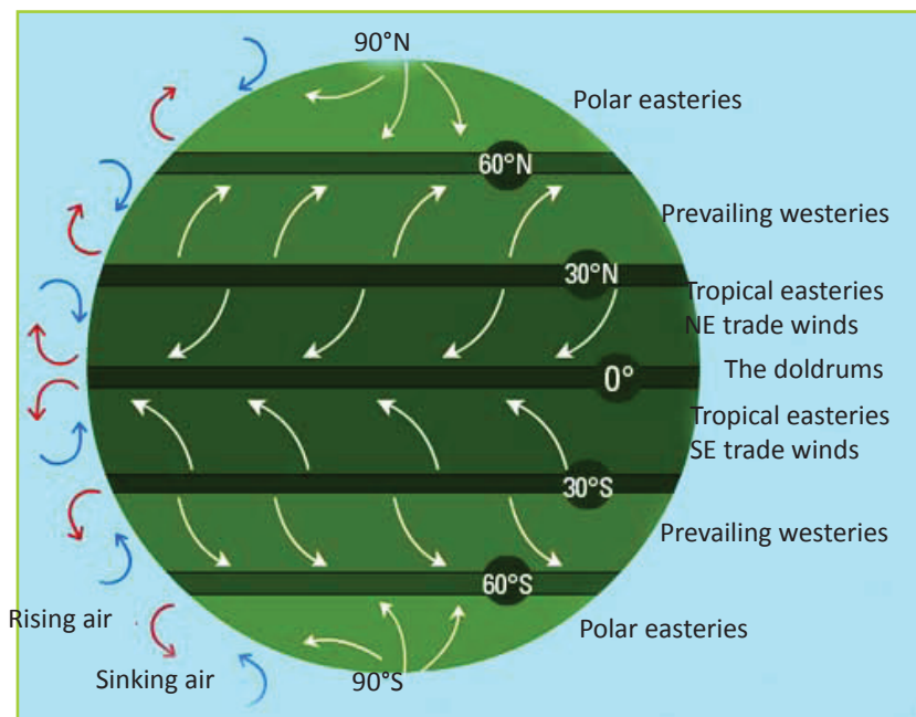
Fig 8.60 Global winds.
