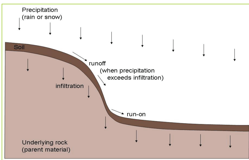
Fig 7.16 Soil catena.
