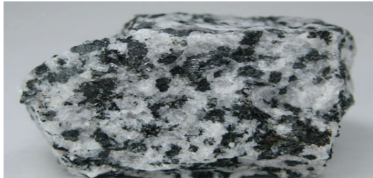
Diorite.
