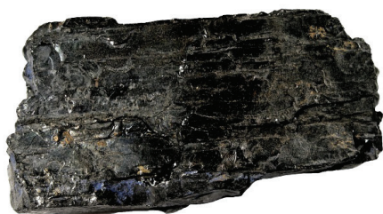
Anthracite coal.
