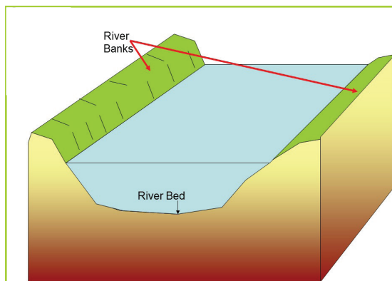
Fig 10.14 A cross profile of a river.
