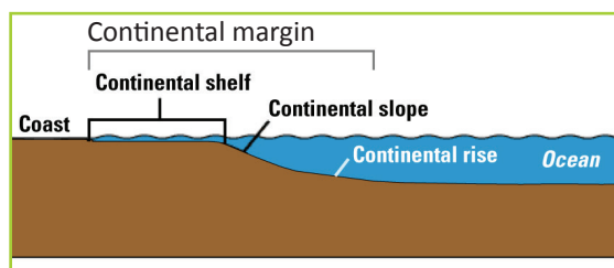
Fig 5.13 Continental shelf.
