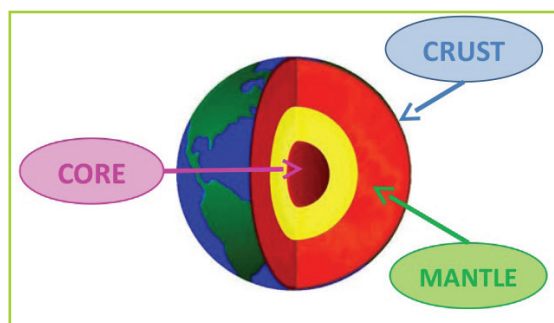
Fig 4.4 The internal structure of the earth.
