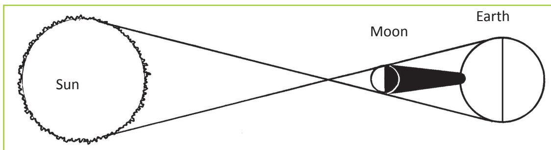
Fig 3.44 (b) An illustration of the solar eclipse.
