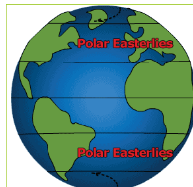
Fig 8.59 Polar easterlies.
