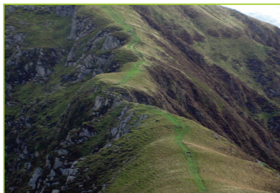
Fig 2. 24 A ridge.
