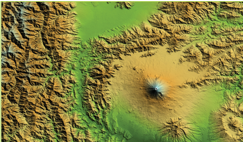
Fig 2.37 Hill shading.
