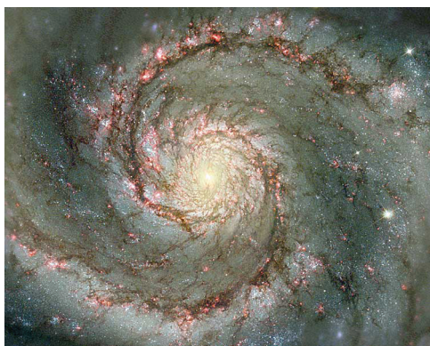
Fig 3.28 The Whirlpool galaxy.
