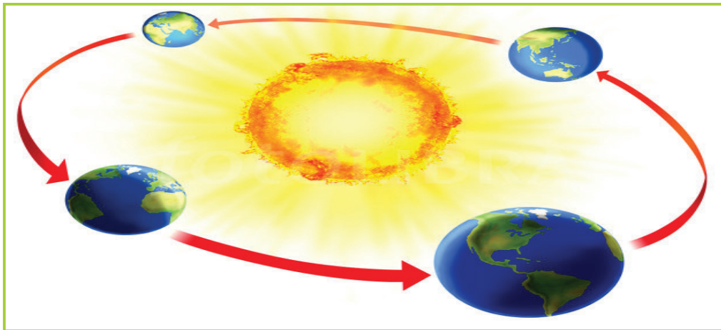
Fig 3.4 The earth orbits the sun.
