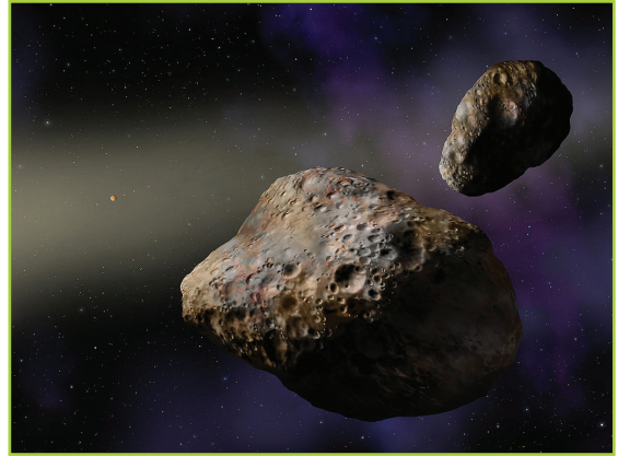
Fig 3.9 Asteroids in space.
