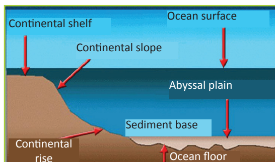
Fig 5.14 Continental slope.
