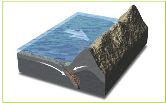
Fig. 11.8 (a) Plates moving towards each other.
