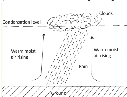
Fig 8.36 Formation of convective rainfall.
