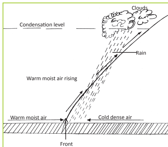
Fig 8.37 Formation of frontal rainfall
