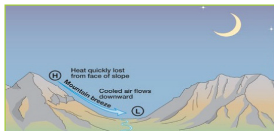
Fig 8.51 Development of a mountain breeze (katabatic winds).
