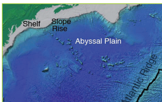
Fig 5.17 Abyssal plain.
