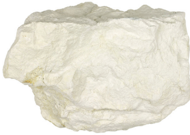
Limestone .
