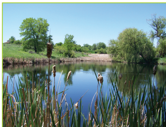
Fig 10.3 A pond.
