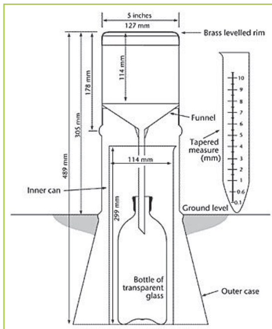
Fig 8.38 The structure of a rain gauge
